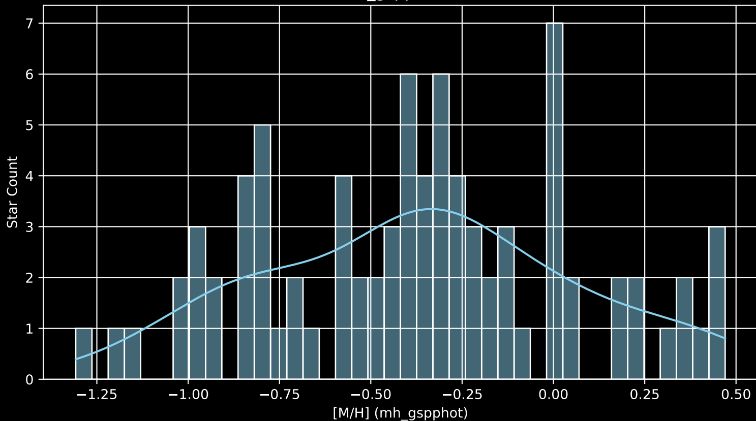
APOGEE DR17 Field: [038+00 [M/H] (mh_gspphot) (n= 83)
