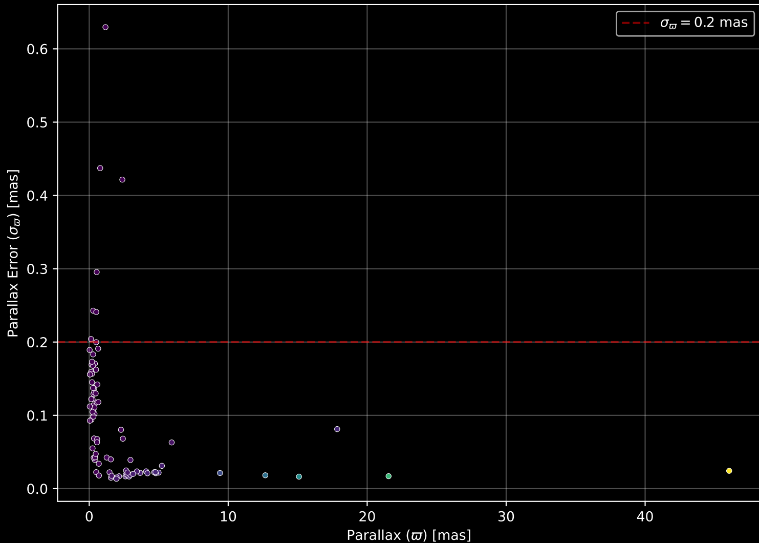
APOGEE DR17 Field: [038+00] Parallax Quality (n= 89)
