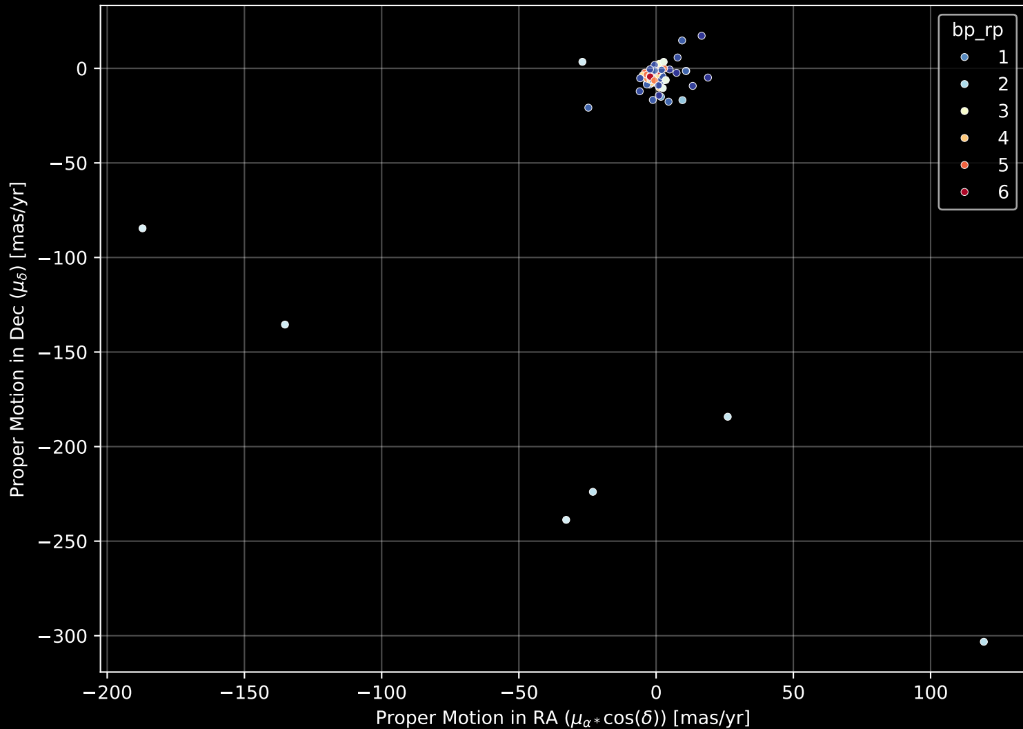
APOGEE DR17 Field: [038+00] Proper Motion Diagram (n= 89)
