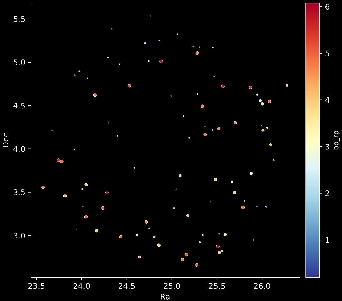
APOGEE DR17 Field: [038+00] Stars: 89
