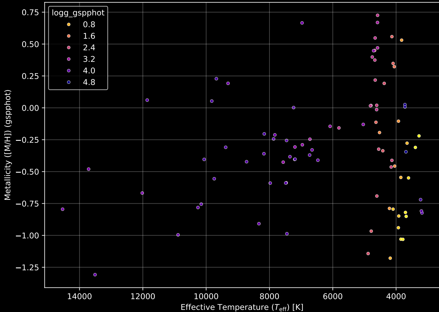
APOGEE DR17 Field: [038+00] Stellar Population Parameters (n= 89)
