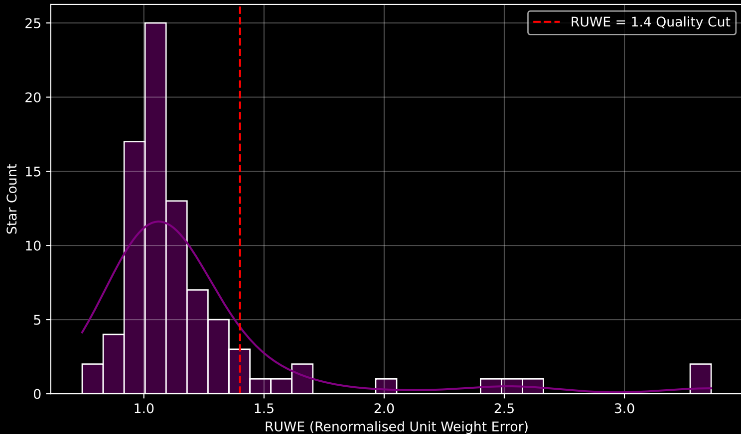
GAPOGEE DR17 Field [038+00] RUWE Distribution (n= 86)
