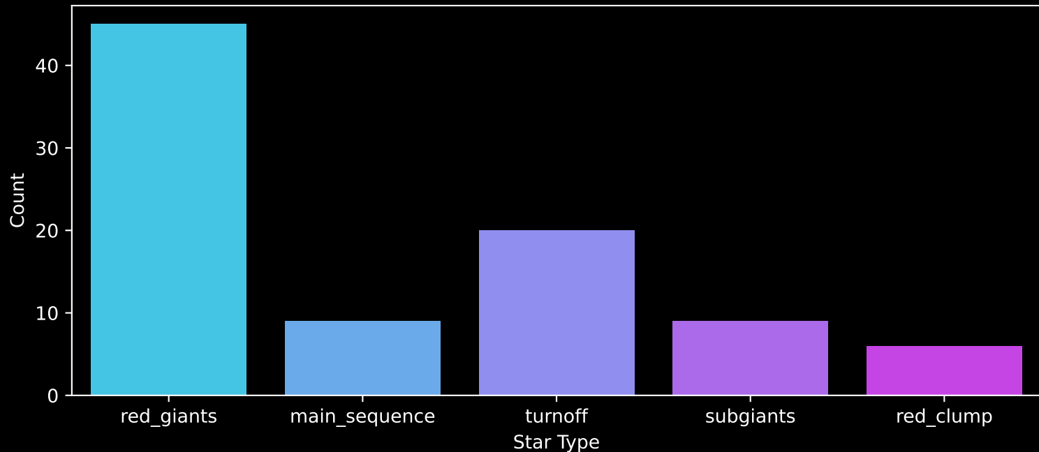
APOGEE DR17 Field: [038+00] Count plot of Star Type
